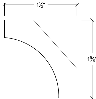
CV2182 11/16" x 2-3/16"
