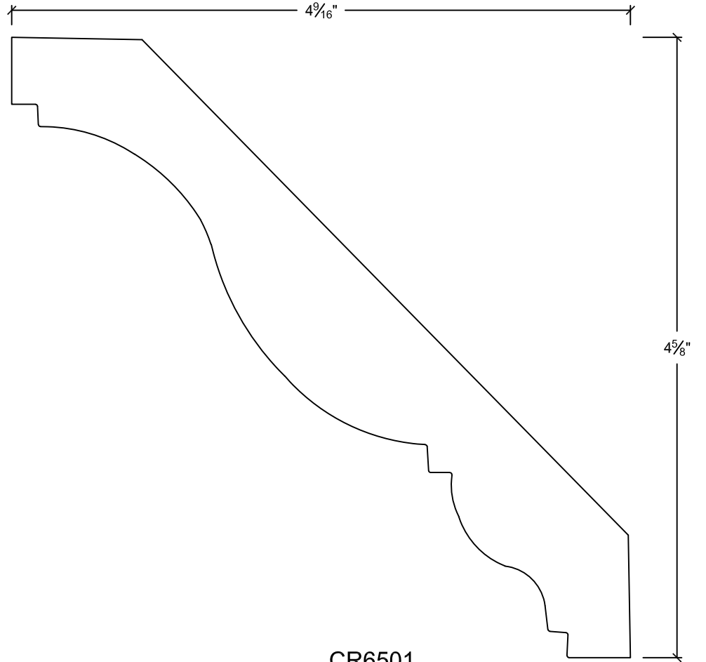
CR6501 1-1/16" x 6-1/2"
