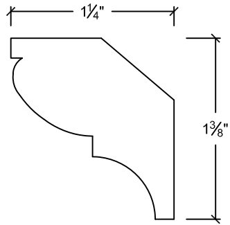
CR1811 13/16" x 1-13/16"
