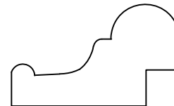
PA1255 3/4" x 1-1/4"
