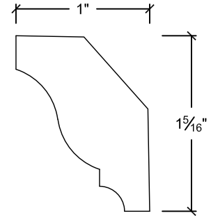
CR1621 5/8" x 1-5/8"
