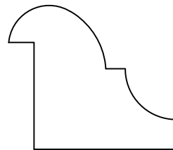
BB1256 1-1/4" x 1-1/16"
