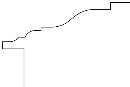
PC2253 1-1/2" x 2-1/4"
