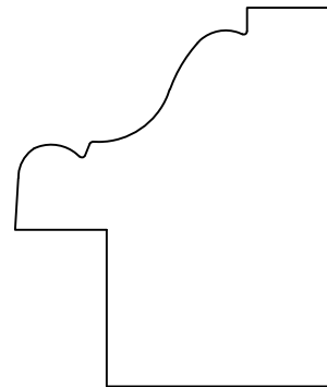
BB1504 1-1/2" x 1-13/16"
