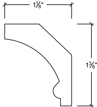
CV1751 3/4" x 1-3/4"
