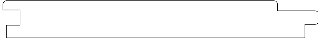
PA5003 1 1/16" x 5-3/4"
