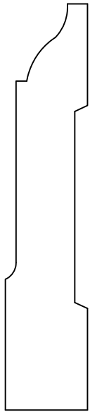
BA3002 5/8" x 3"
