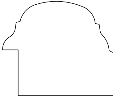
BB1872 1-7/8" x 1-9/16"
