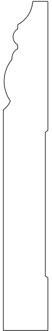
BA5501 3/4" x 5-1/2"
