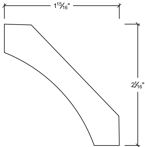
CV2812 5/8" x 2-13/16"
